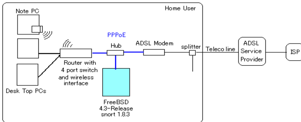
Figure 1 ADSL Home User Configuration
