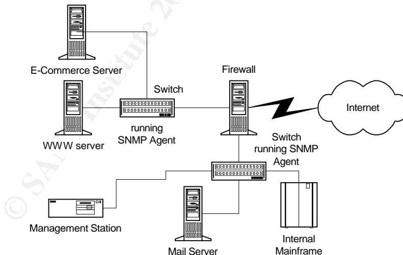
Diagram 2. SNMP Management Station
