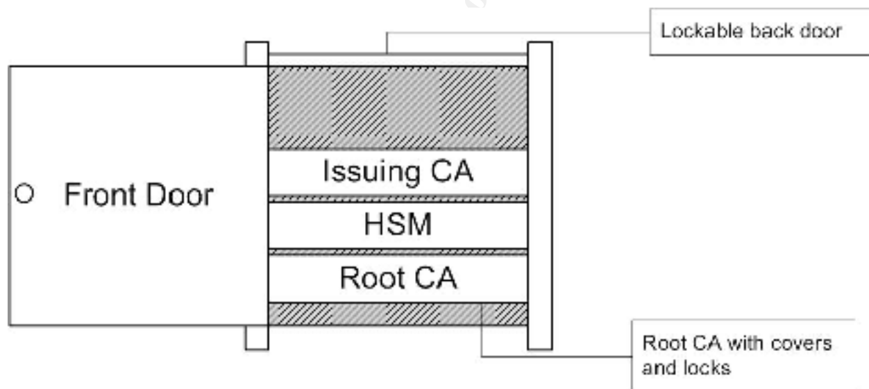
Figure 2: Rack Illustration
