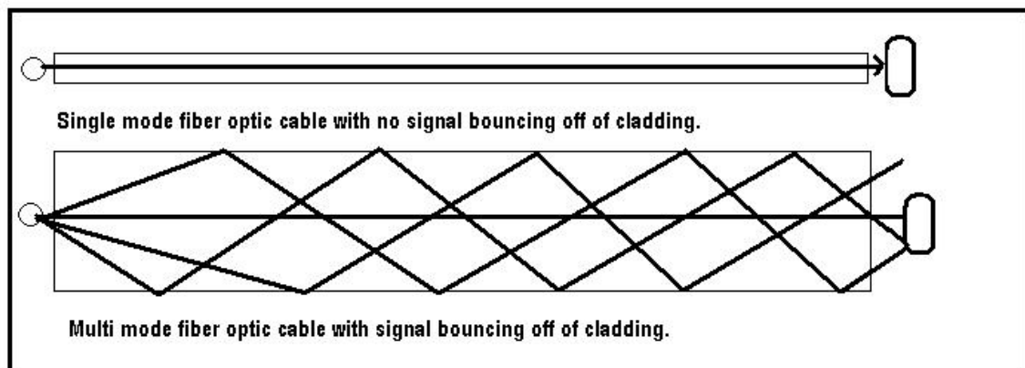
Difference between Single mode and Multi mode fiber optic cable.
