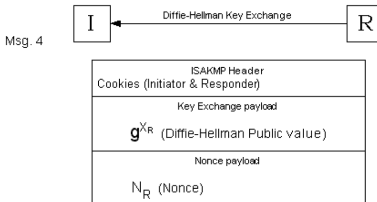
Figure 6b. ISAKMP round trip #2 (message 4)
